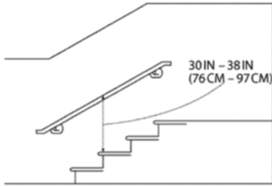
Figure D-12 – Handrail Measurement
