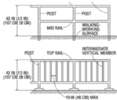
Figure D-11 – Guard Rail Systems
