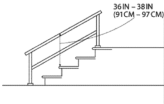
Figure D-13 - Combination Handrail and Stair Rail
